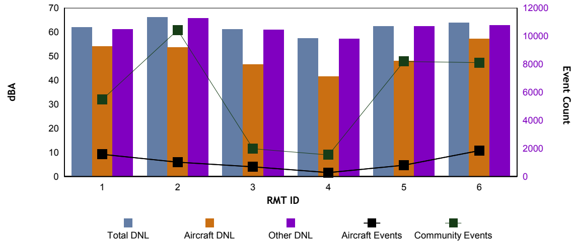
Noise Distribution
